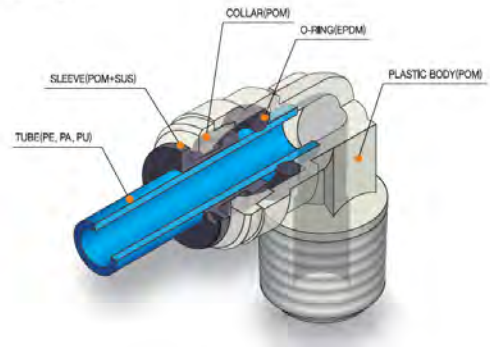
Structural Diagram
