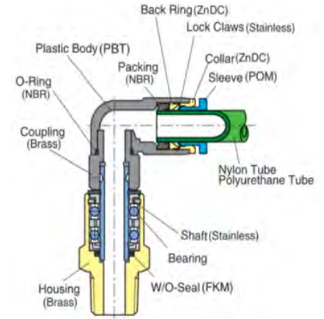
Rotary Joint
