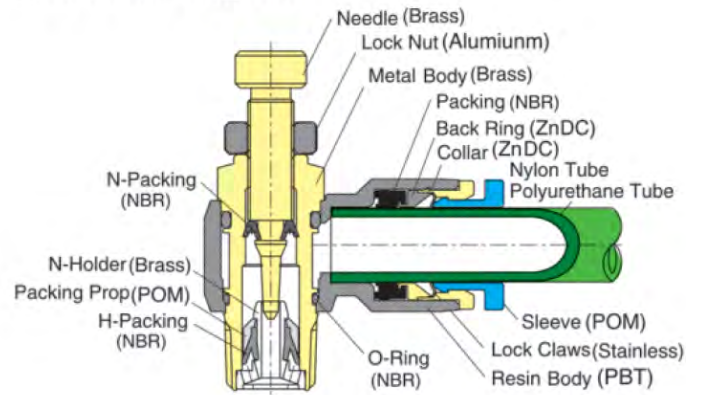
Structural Diagram
