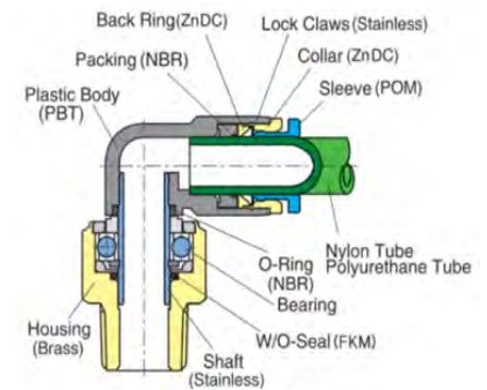
Rotary Joint
