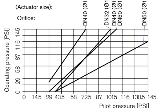
Chart 4 - orifice 1 1/4"-2"
