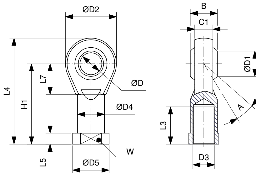
SELF-LUBRICATING SPHERICAL ROD ENDS
