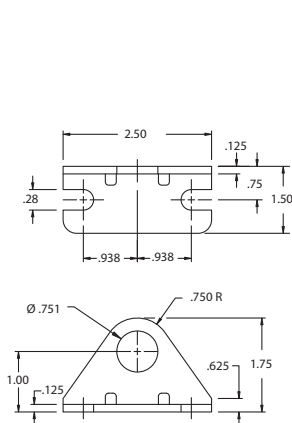
Mounting Bracket F-M117007 Price: $3.57
