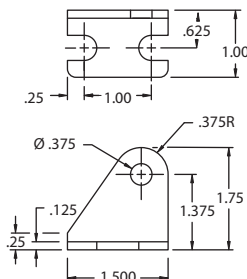
Pivot Bracket F-M029004 Price: $5.24
