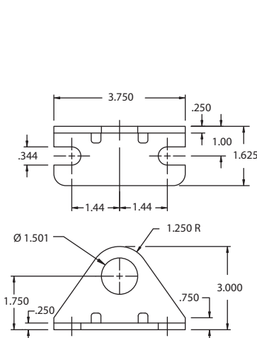
Mounting Bracket F-M117010 Price: $20.46
