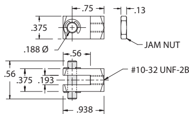
Rod Clevis F-M127002 Price: $3.05
