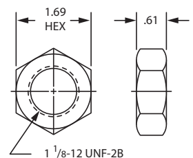
Mounting Nut F-M190015 Price: $4.45
