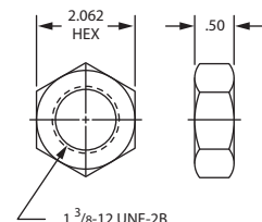
Mounting Nut F-M190012 Price: $5.74
