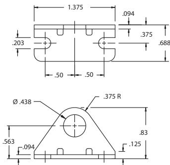
Mounting Bracket F-M117003 Price: $1.92
