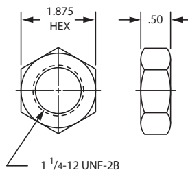
Mounting Nut F-M190009 Price: $3.64
