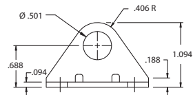
Mounting Bracket F-M117006 Price: $2.12
