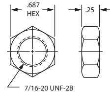
Mounting Nut F-M190003 Price: $0.26
