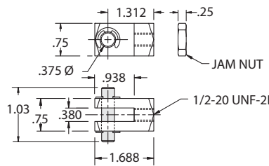
Rod Clevis F-M127006 Price: $5.80
