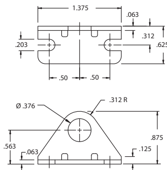
Mounting Bracket F-M117004 Price: $1.92
