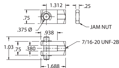
Rod Clevis F-M127005 Price: $5.80
