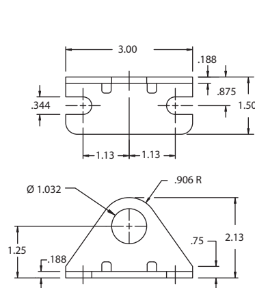
Mounting Bracket F-M117008 Price: $5.80
