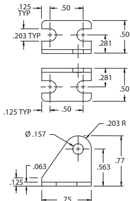
Pivot Bracket F-M029002 Price: $3.05
