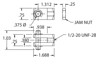
Rod Clevis F-M127006 Price: $5.80
