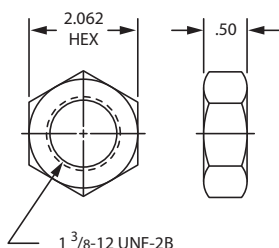
Mounting Nut F-M190012 Price: $5.74
