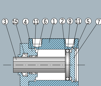
Single Rod/Nonrotating
