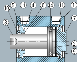
Single Rod/Double Acting Rear Boss Mount
