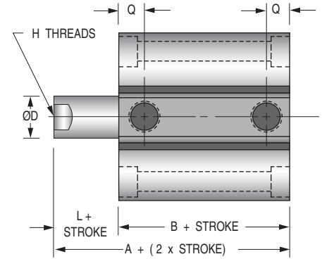
Spring Extend
