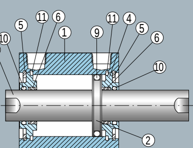
Double Rod/Double Acting
