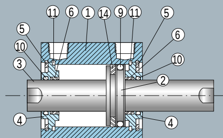
Double Rod/Double Acting
