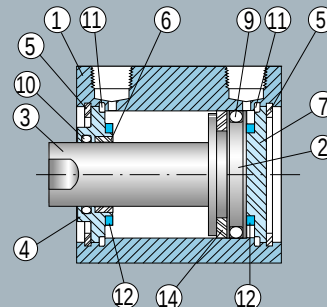
Single Rod/Double Acting Bumpers Front and Rear
