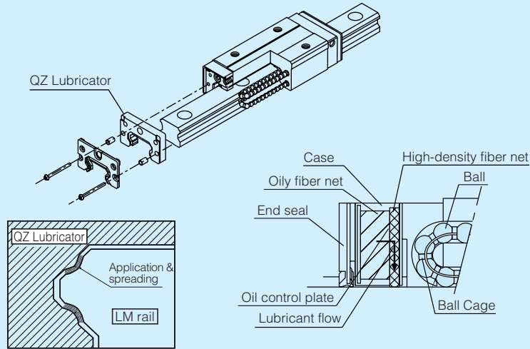
Figure 8 QZ Lubricator Structure Diagram (LM Guide)
