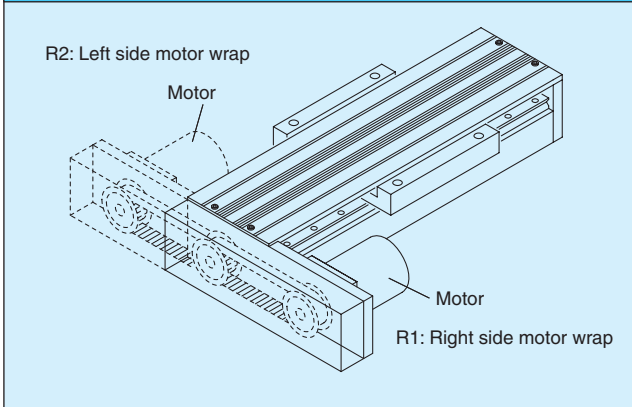
Axial dimensions are kept to minimum by applying the Wrap-Around option. (Pulley ratio: 1:1)
