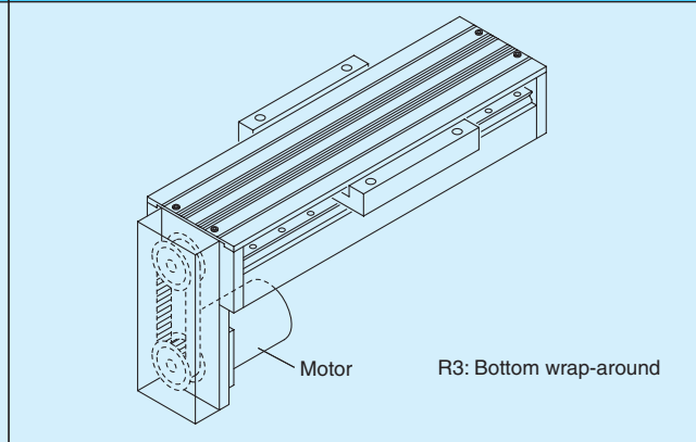
When horizontal space is at a minimum, the bottom side Wrap-Around option is available. (Pulley ratio: 1:1)
