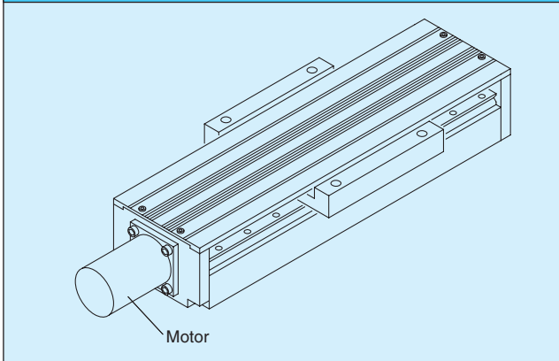
Direct mounting of Motor to Ball Screw.
